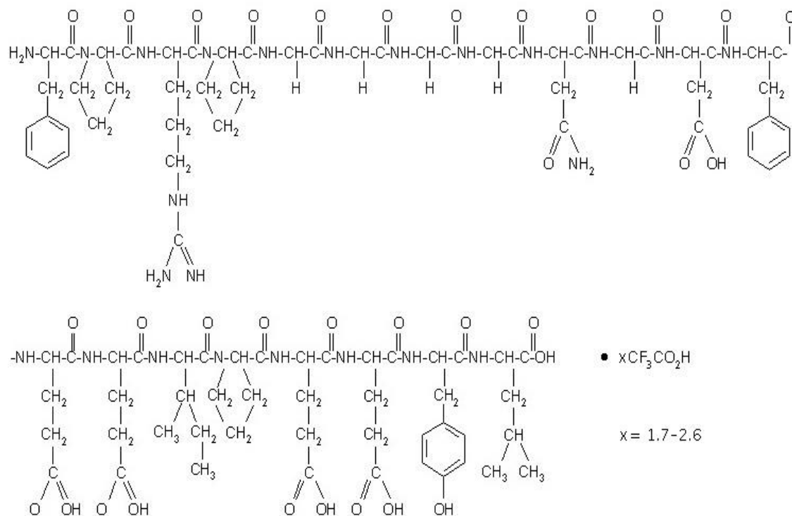
Figure 1: Structure formula for bivalirudin trifluoroacetate
